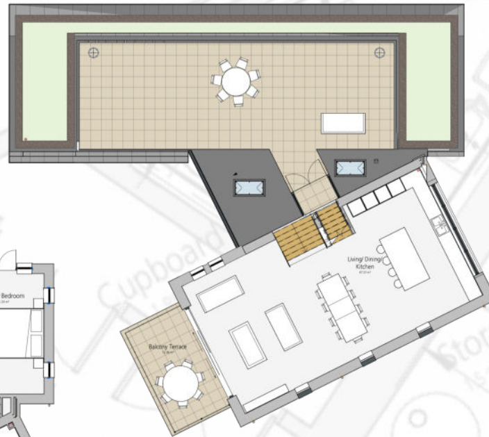
TRESCO FIRST FLOOR
