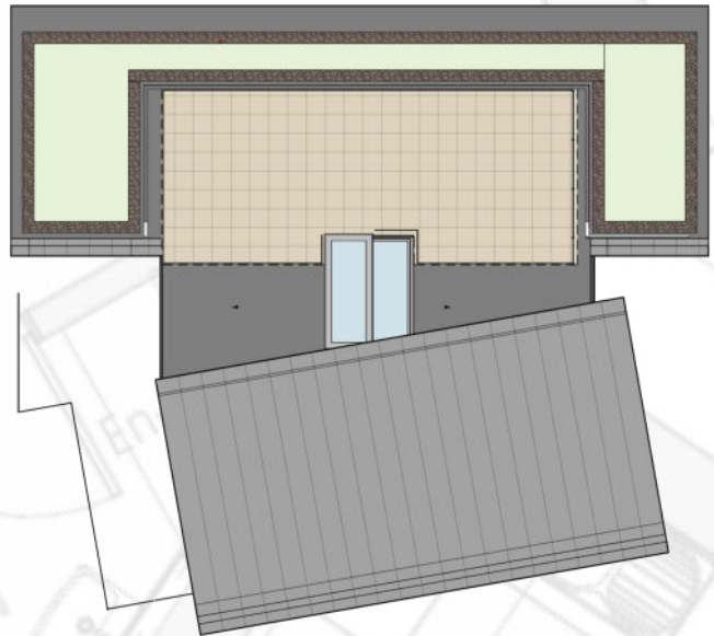
TRERICE ROOF PLAN
