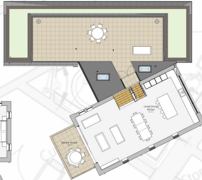
TREGOTHNAN FIRST FLOOR
