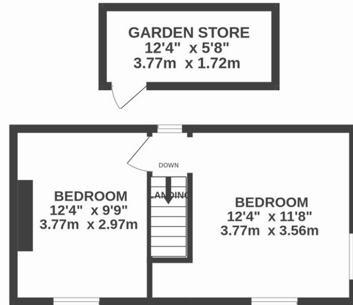
1ST FLOOR 295 sq.ft. (27.4 sq.m.) approx.
