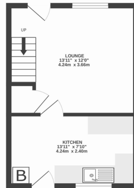
GROUND FLOOR 276 sq.ft. (25.7 sq.m.) approx.
