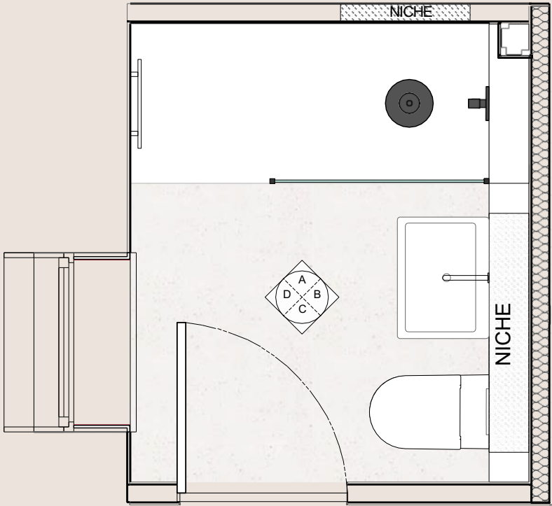
FLOOR PLAN
