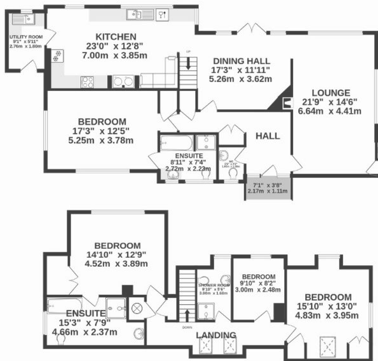
TOTAL FLOOR AREA : 2985 sq.ft. (277.3 sq.m.) approx.
