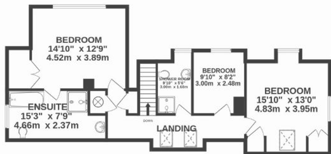
TOTAL FLOOR AREA : 2985 sq.ft. (277.3 sq.m.) approx.
